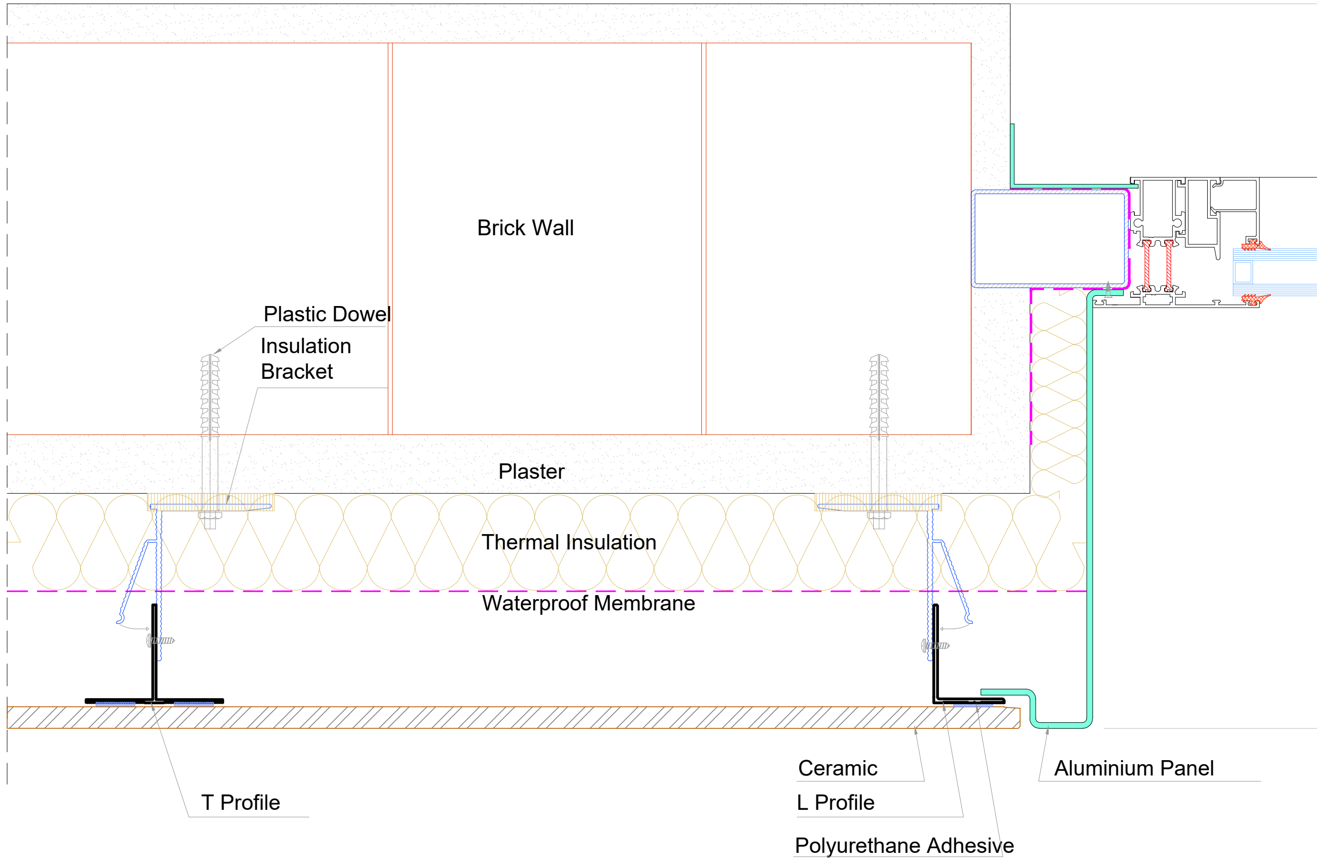
DETAIL 7
