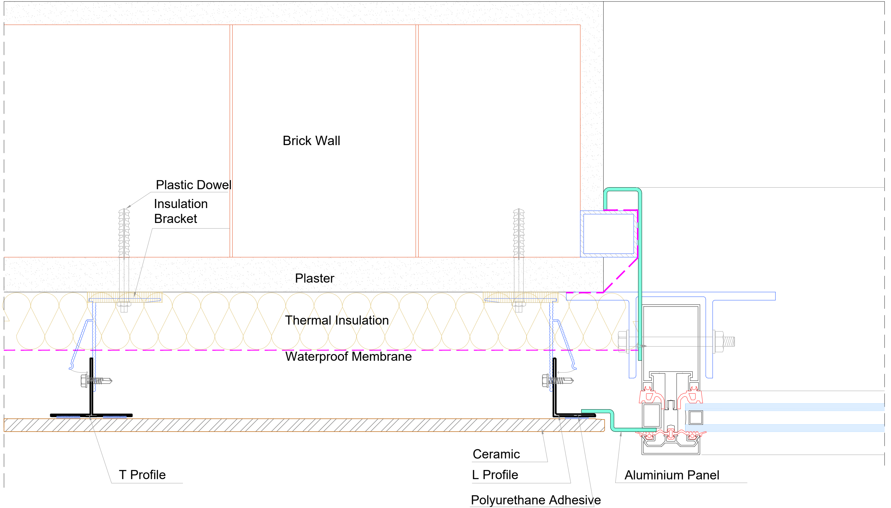
DETAIL A
